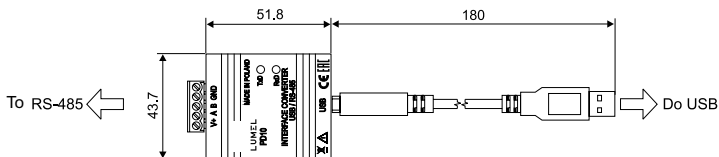
Fig.1 Overall dimensions of the PD10 converter
